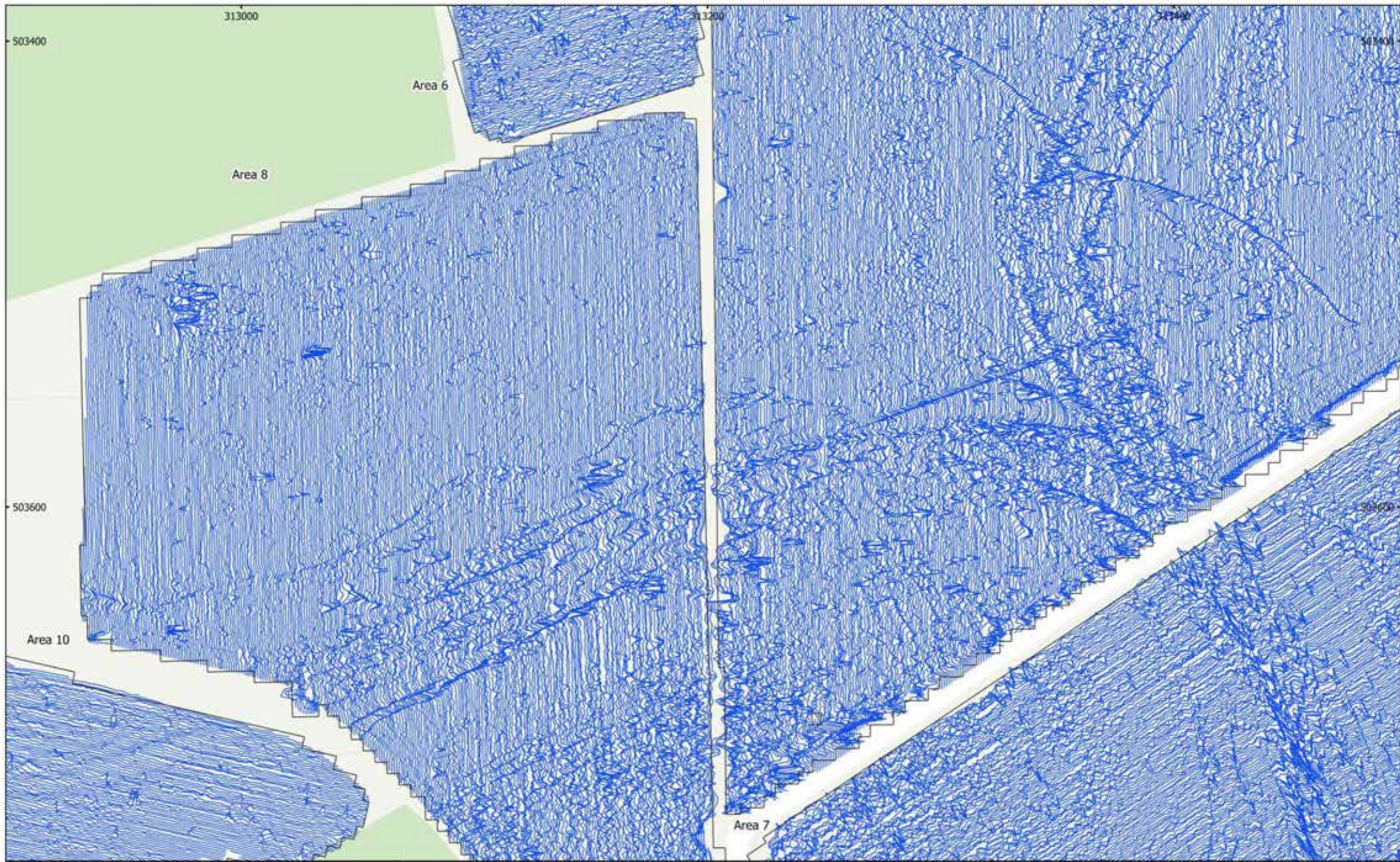
MSTF1136: Mallard Pass, DCO, Essendine, Rutland Figure 56 - XY Trace Plot (Areas 6, 7, 8 & 10) 30nT/cm at 1:1,500 @ A3 Copyright Magnitude Surveys Ltd 2022 Contains Ordnance Survey data © Crown Copyright and database right 2022
