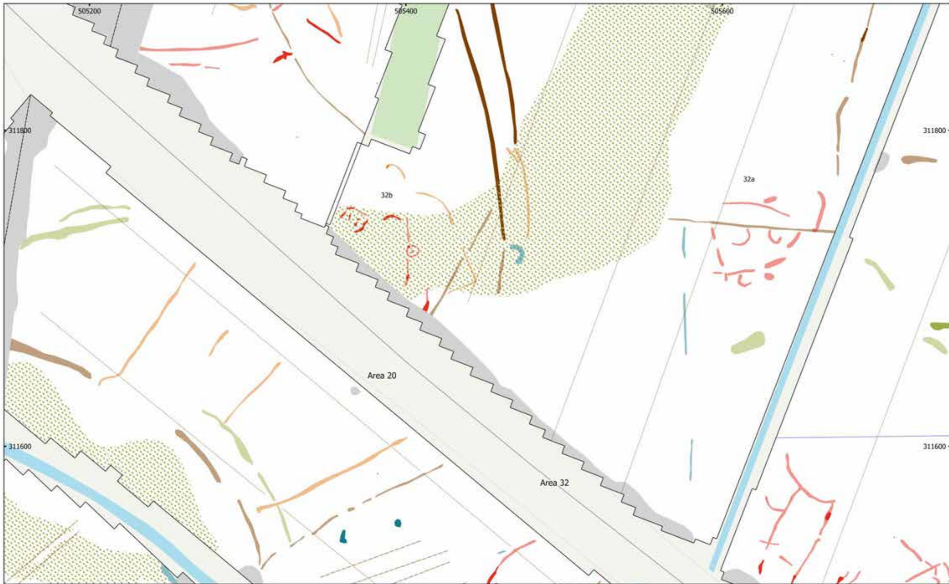
MSTF1136: Mallard Pass, DCO, Essendine, Rutland Figure 127 - Magnetic Interpretation (Areas 20, 27, 32 & 35) 1:1,500 @ A3 Copyright Magnitude Surveys Ltd 2022 Contains Ordnance Survey data © Crown Copyright and database right 2022
