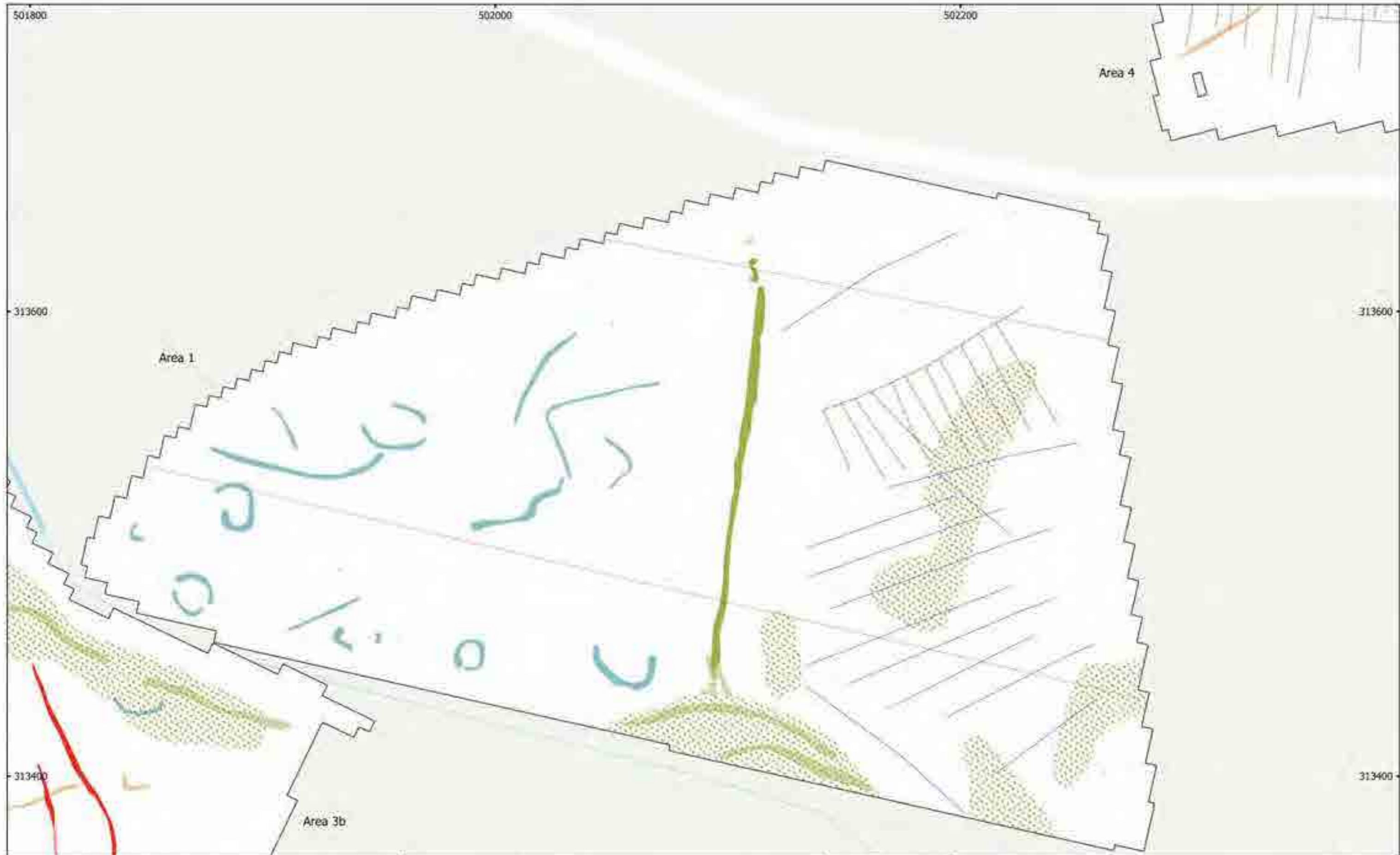
MSTF1136- Mallard Pass, DCO, Essendine, Rutland Figure 40 - Magnetic Interpretation (Area 1 & 3b) 1:1,500 @ A3 Copyright Magnitude Surveys Ltd 2022 Contains Ordnance Survey data © Crown Copyright and database right 2022
