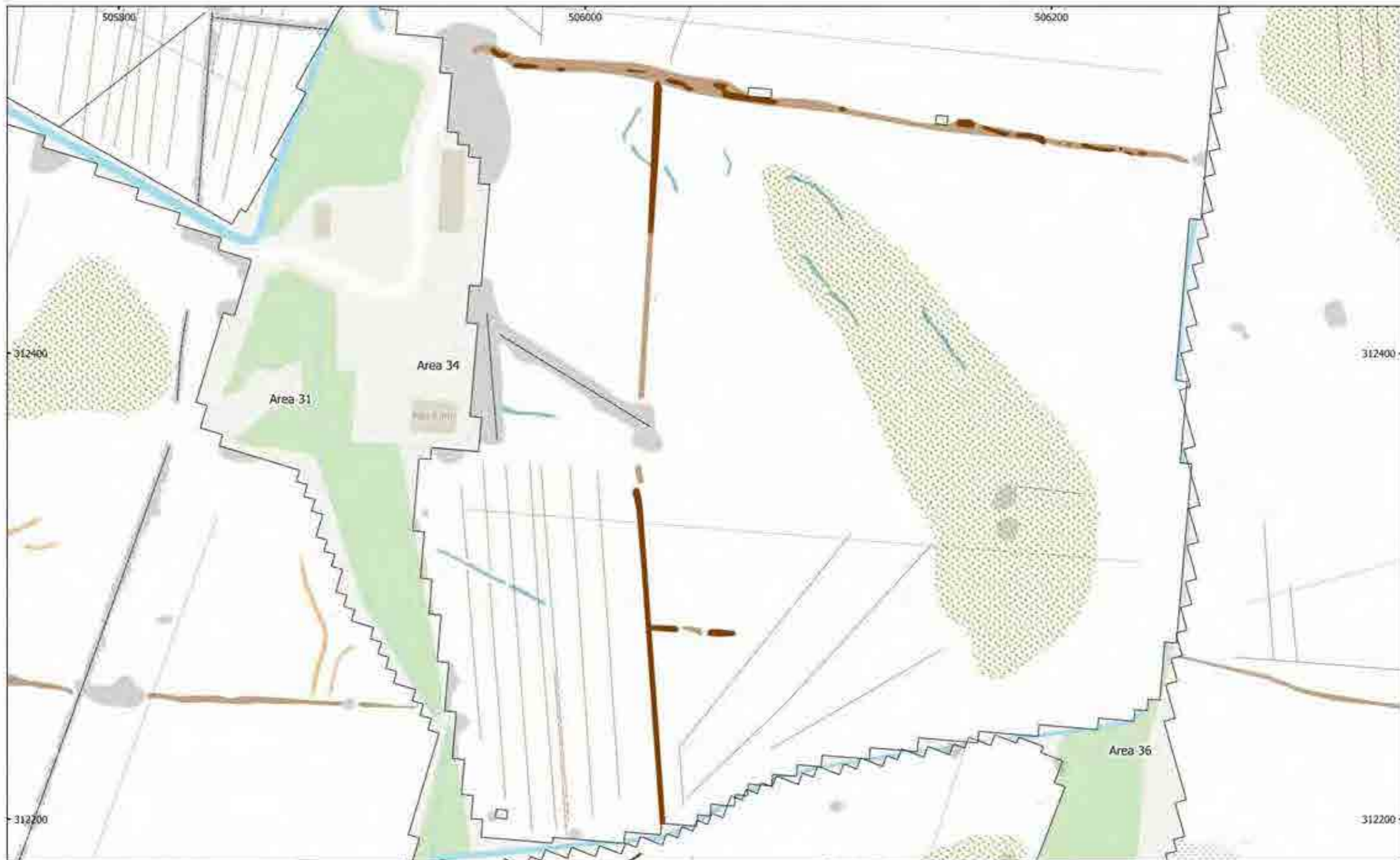
MSTF1136- Mallard Pass, DCO, Essendine, Rutland Figure 106 - Magnetic Interpretation (Areas 31, 34 & 36) 1:1,500 @ A3 Copyright Magnitude Surveys Ltd 2022 Contains Ordnance Survey data © Crown Copyright and database right 2022
