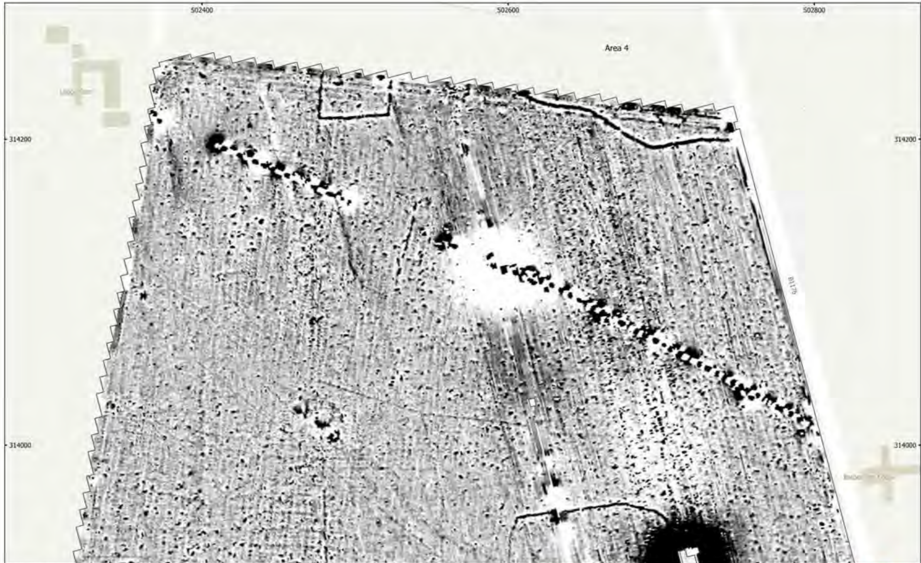
M5TF1136: Mallard Pass, DCO, Essendine, Rutland Figure 42 - Magnetic Gradient (Area 4 (North)) 1:1,500 @ A3 Copyright Magnitude Surveys Ltd 2022 Contains Ordnance Survey data © Crown Copyright and database right 2022
