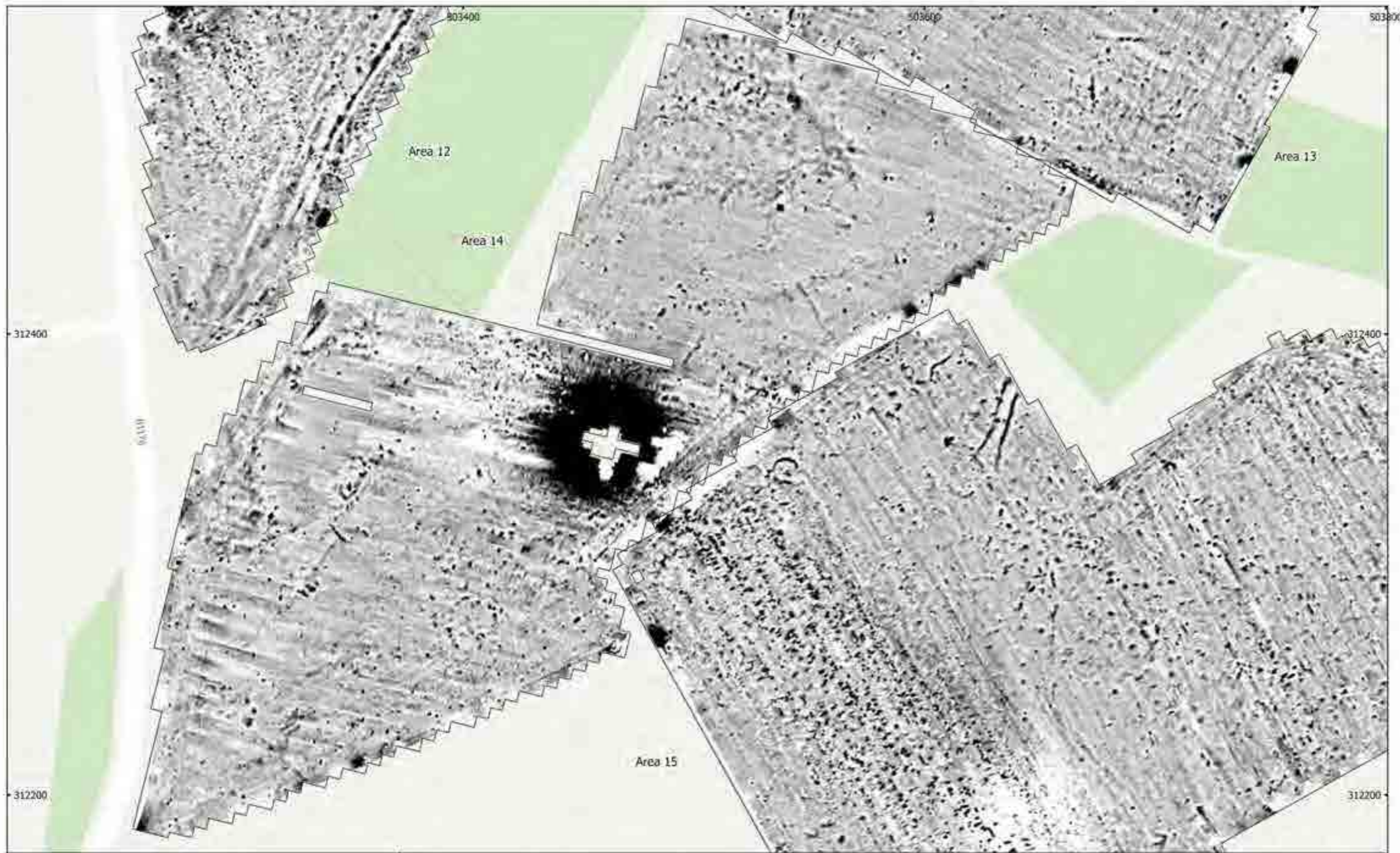
MSTF1136: Mallard Pass, DEO, Essendine, Rutland Figure 75 - Magnetic Gradient (Areas 12, 13, 14 & 15.) 1:1,500 @ A3 Copyright Magnitude Surveys Ltd 2022 Contains Ordnance Survey data © Crown Copyright and database right 2022
