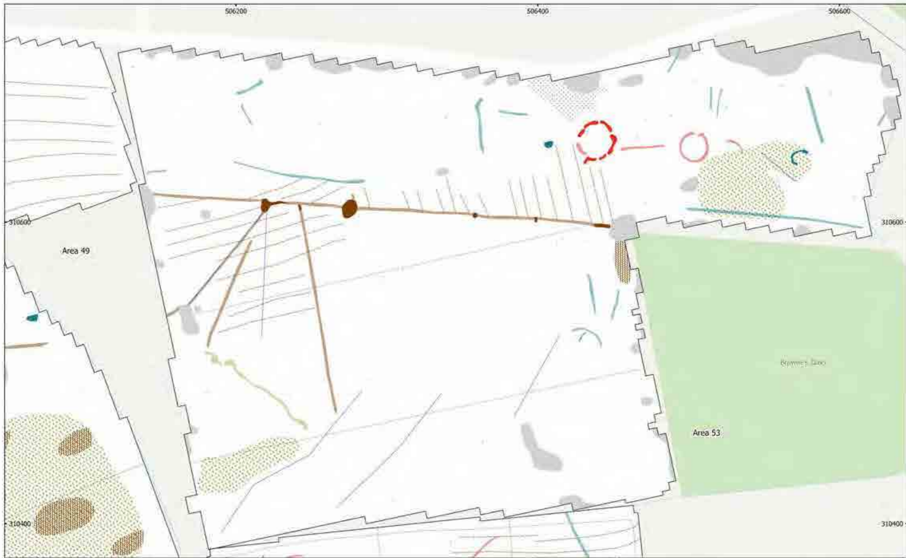
MSTP1136- Mallard Pass, DCO, Essendine, Rutland Figure 157 - Magnetic Interpretation (Areas 49 & 53) 1:1,500 @ A3 Copyright Magnitude Surveys Ltd 2022 Contains Ordnance Survey data © Crown Copyright and database right 2022
