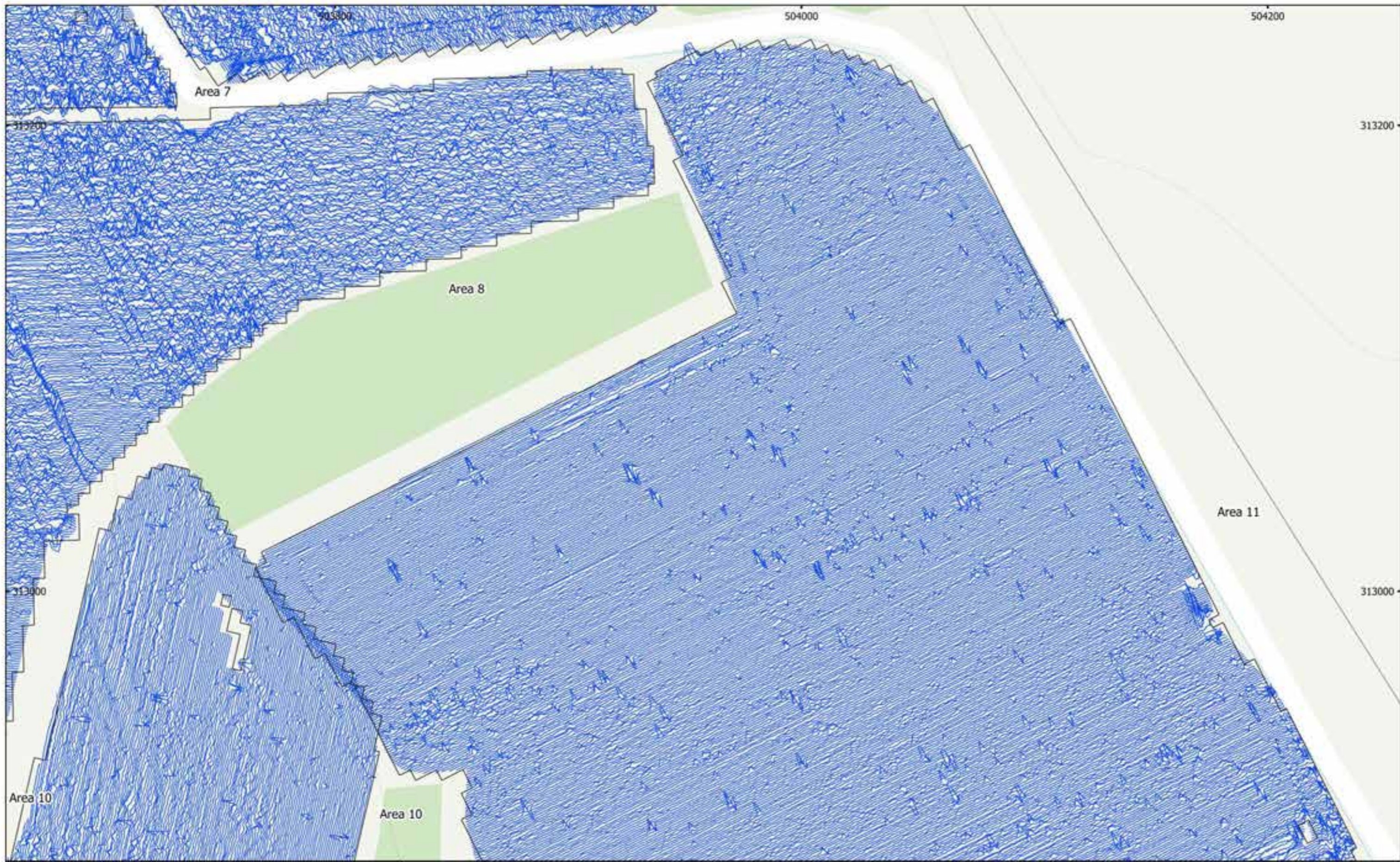
MSTF1136: Mallard Pass, DCO, Essendine, Rutland Figure 68 - XY Trace Plot (Areas 8, 10 & 11) 30nT/cm at 1:1,500 @ A3 Copyright Magnitude Surveys Ltd 2022 Contains Ordnance Survey data © Crown Copyright and database right 2022
