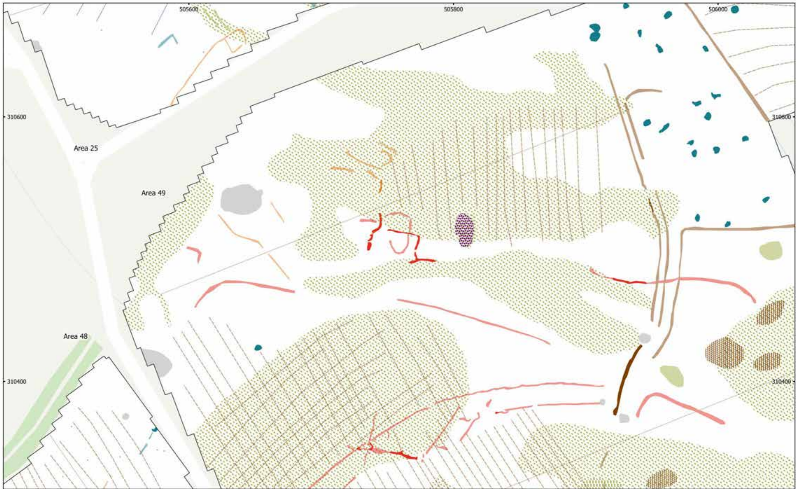
MSTF1136: Mallard Pass, DCO, Essendine, Rutland Figure 154 - Magnetic Interpretation (Areas 25 & 49) 1:1,500 @ A3 Copyright Magnitude Surveys Ltd 2022 Contains Ordnance Survey data © Crown Copyright and database right 2022
