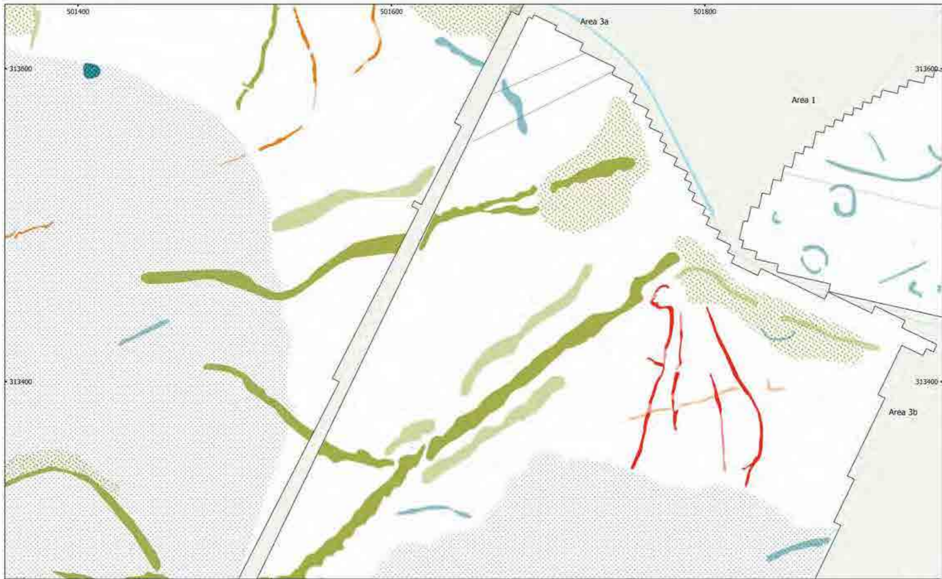
MSTP1136: Mallard Pass, DCO, Essendine, Rutland Figure 34 - Magnetic Interpretation (Areas 1, 3a & 3b) 1:1,500 @ A3 Copyright Magnitude Surveys Ltd 2022 Contains Ordnance Survey data © Crown Copyright and database right 2022
