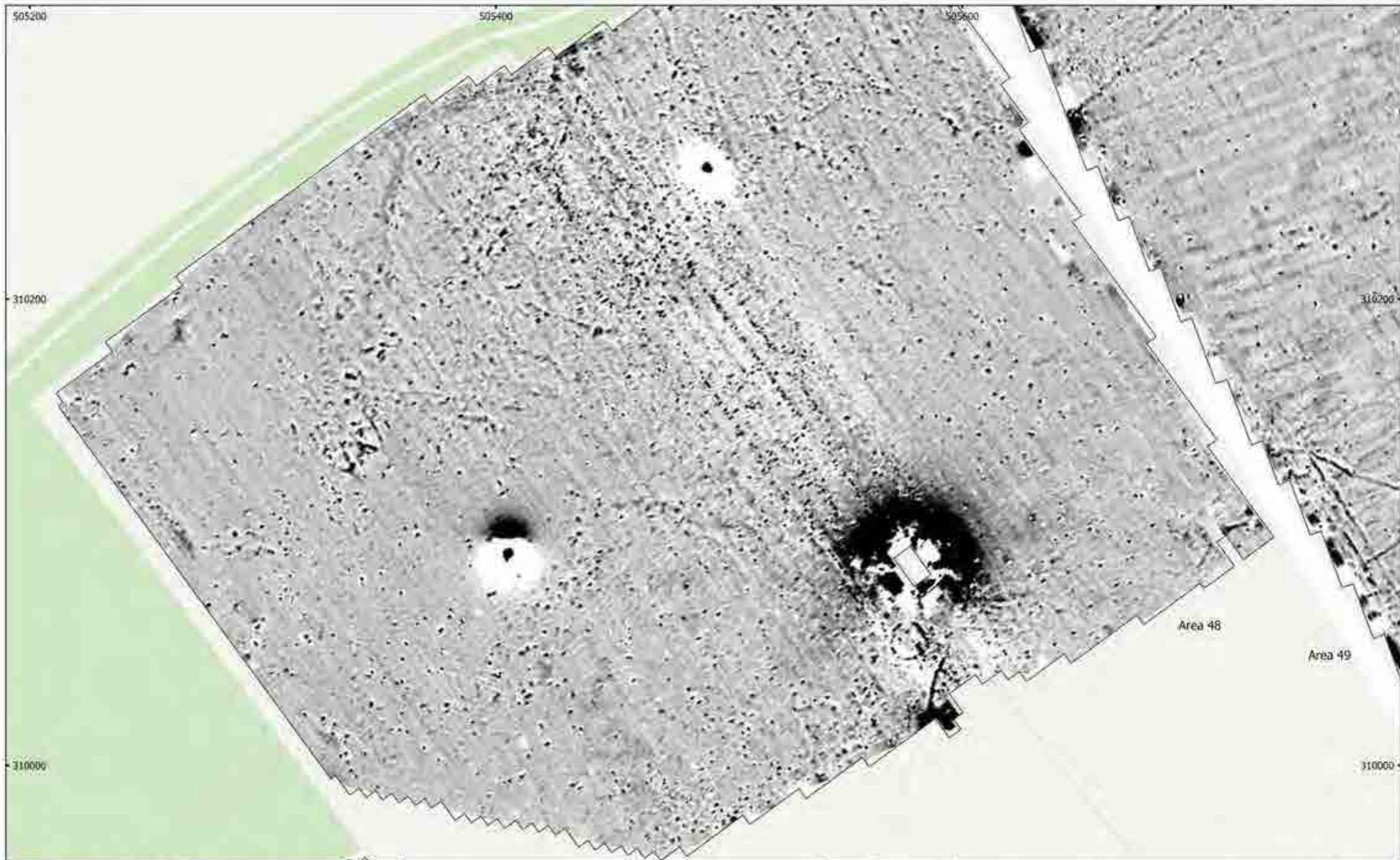
MSTP1136: Mallard Pass, DCO, Essendine, Rutland Figure 159 - Magnetic Gradient (Areas 48 & 49) 1:1,500 @ A3 Copyright Magnitude Surveys Ltd 2022 Contains Ordnance Survey data © Crown Copyright and database right 2022
