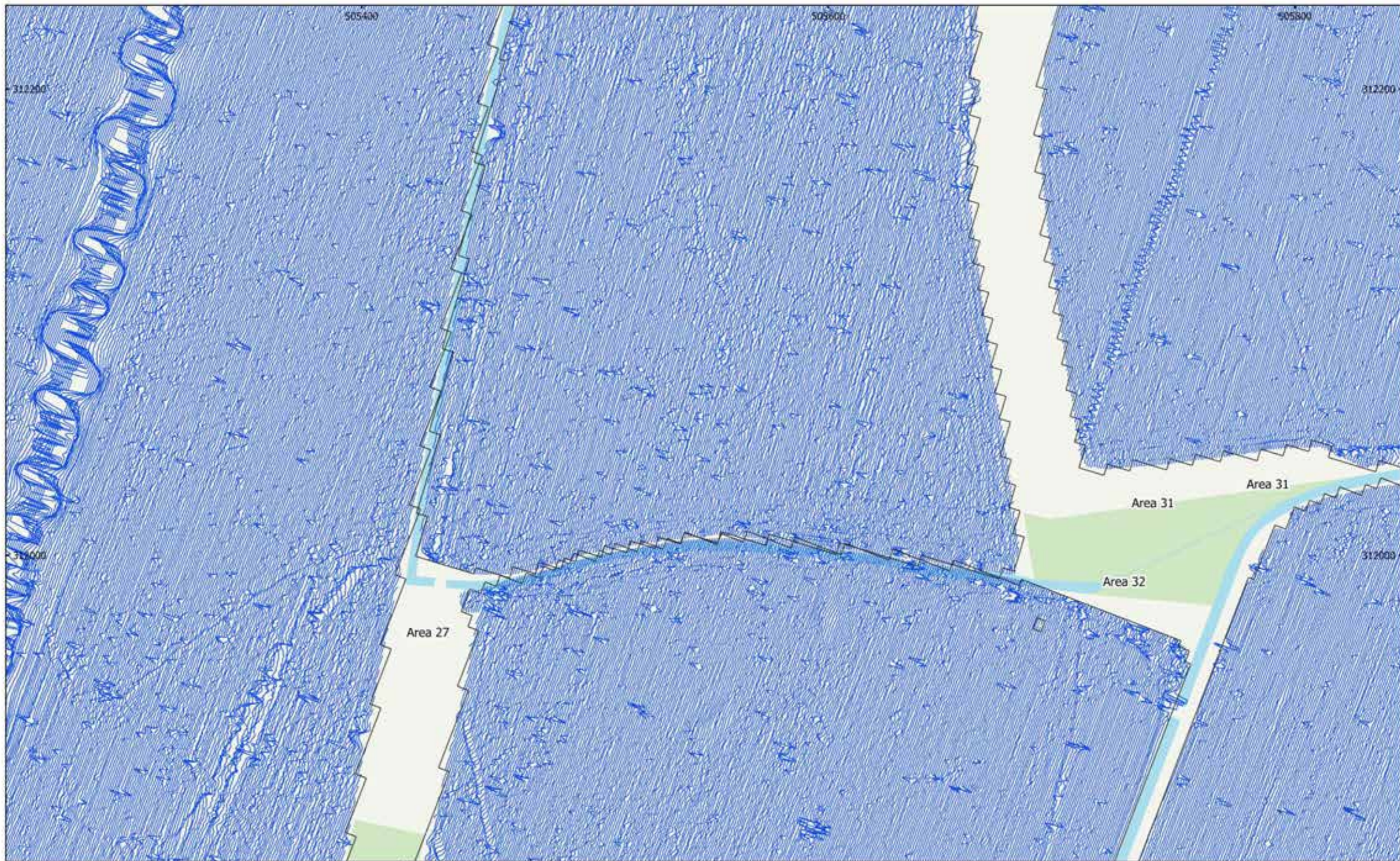
MSTF1136: Mallard Pass, DCO, Essendine, Rutland Figure 116 - XY Trace Plot (Areas 27, 31 & 32) 30nT/cm at 1:1,500 @ A3 Copyright Magnitude Surveys Ltd 2022 Contains Ordnance Survey data © Crown Copyright and database right 2022
