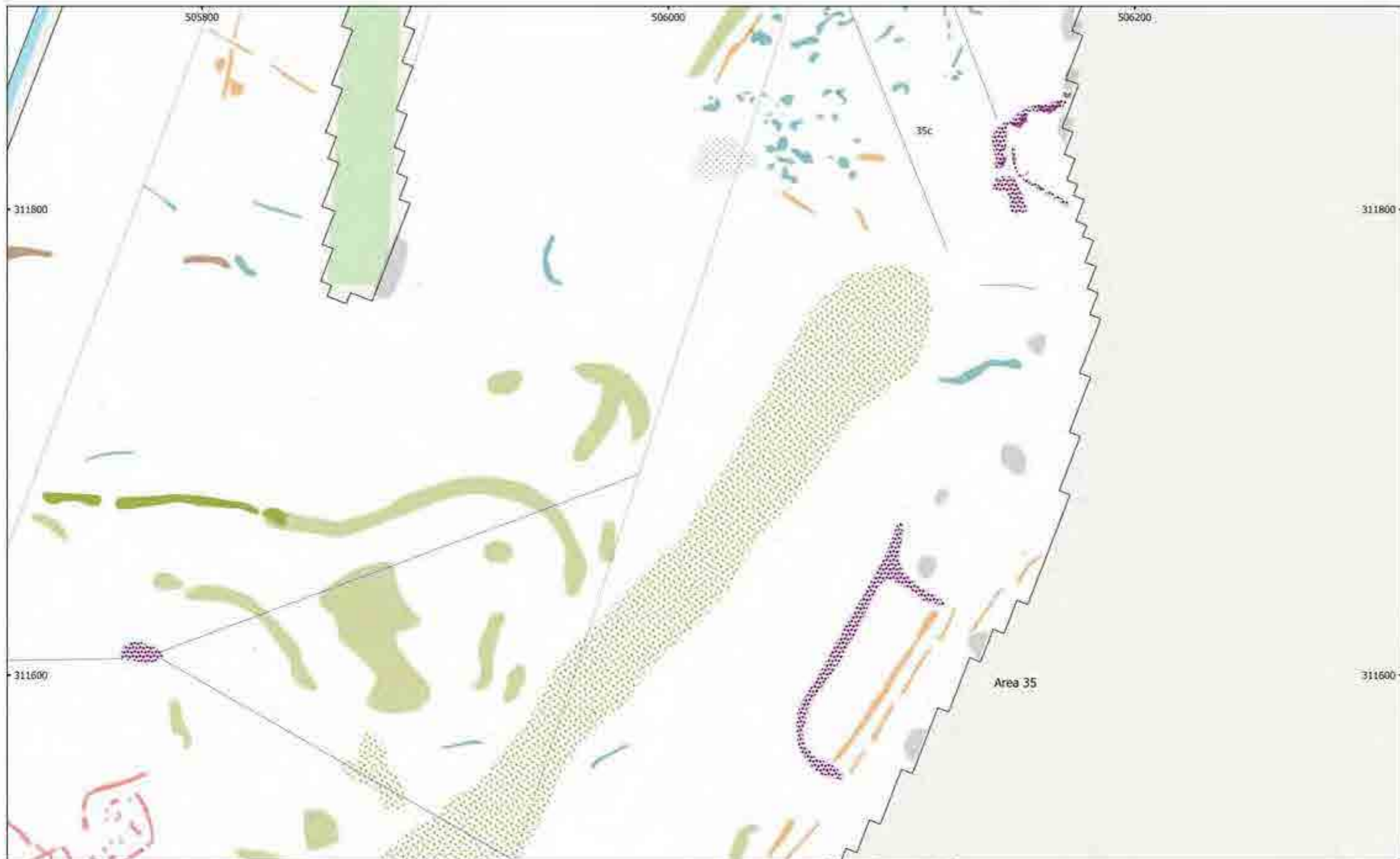
MSTF1136: Mallard Pass, DCO, Essendine, Rutland Figure 130 - Magnetic Interpretation (Area 35 (Central)) 1:1,500 @ A3 Copyright Magnitude Surveys Ltd 2022. Contains Ordnance Survey data © Crown Copyright and database right 2022
