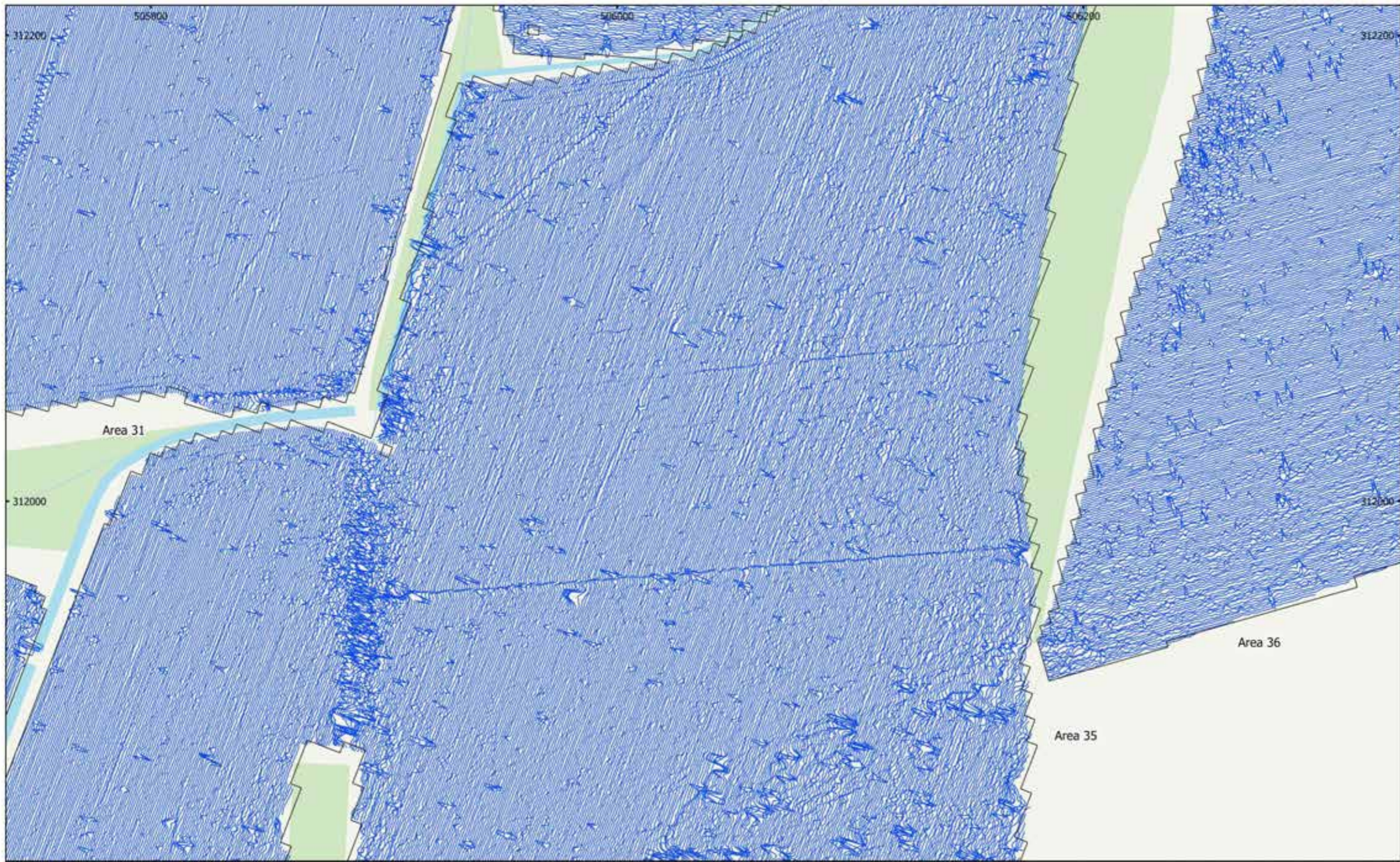
MSTF1136: Mallard Pass, DCO, Essendine, Rutland Figure 119 - XY Trace Plot (Areas 31, 35 & 36) 30nT/cm at 1:1,500 @ A3 Copyright Magnitude Surveys Ltd 2022 Contains Ordnance Survey data © Crown Copyright and database right 2022
